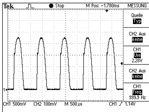
Figure 3: The demodulated 1 kHz disturbance signal is limited by the lower rail.
