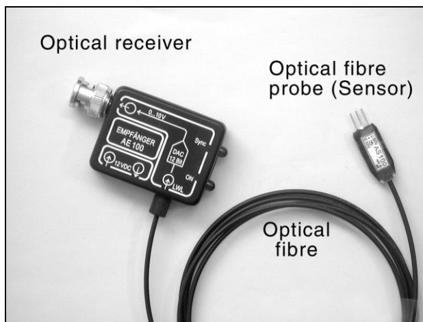
Figure 7: Optical fibre measuring system
