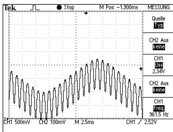
Figure 5: Useful signal with 1 kHz disturbance signal
