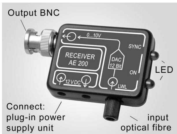
Figure 10: AE 200 connectors and displays
