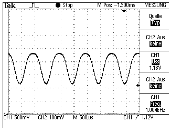
Figure 1: The oscillogram shows a constant useful signal with a demodulated 1 kHz component.
