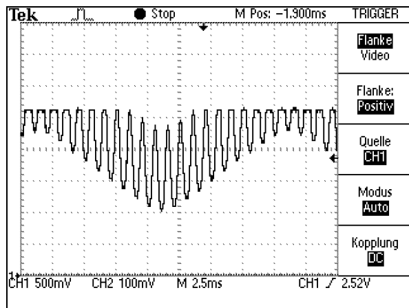
Figure 6: Useful signal with 1 kHz disturbance signal limited by the upper rail
