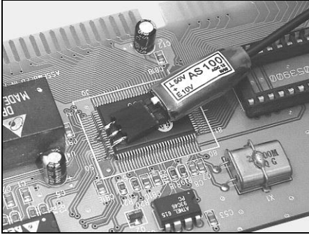
Figure 9: AS 100 is connected to the EUT; position the AS 100 on the IC package if there isn't enough free space above GND
