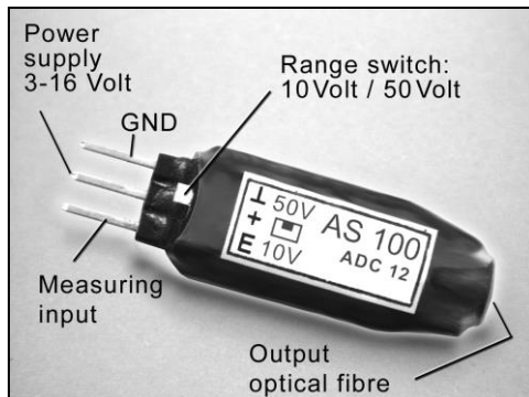
Figure 8: AS 100 pin assignment
