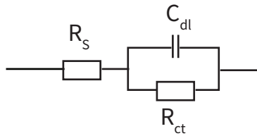
Model of simplified Randles cell
