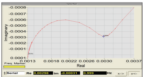
Nyquist diagram
