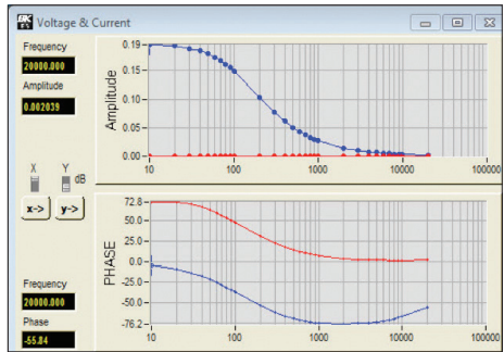
V/I plot
