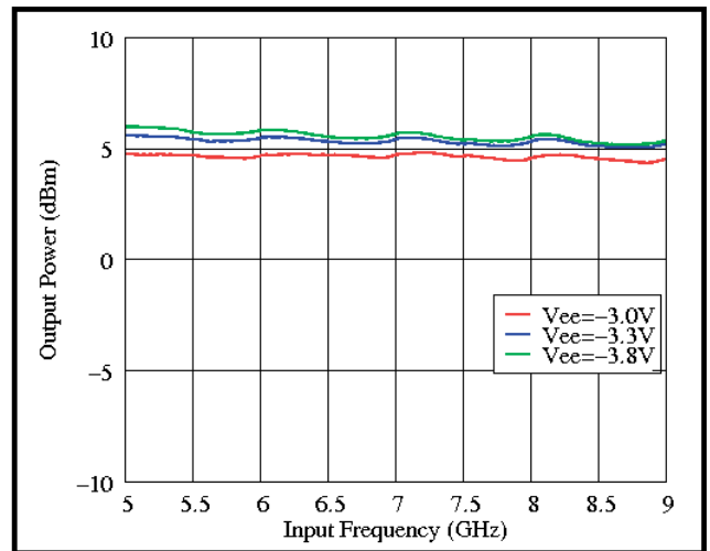
Output Power Divide-by-10, FRS=1
