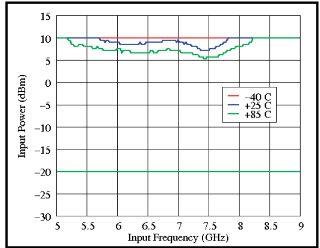
Min/Max Single-Ended Input Power, INP* Input Sensitivity, -3.3, Divide-by-10, FRS=1
