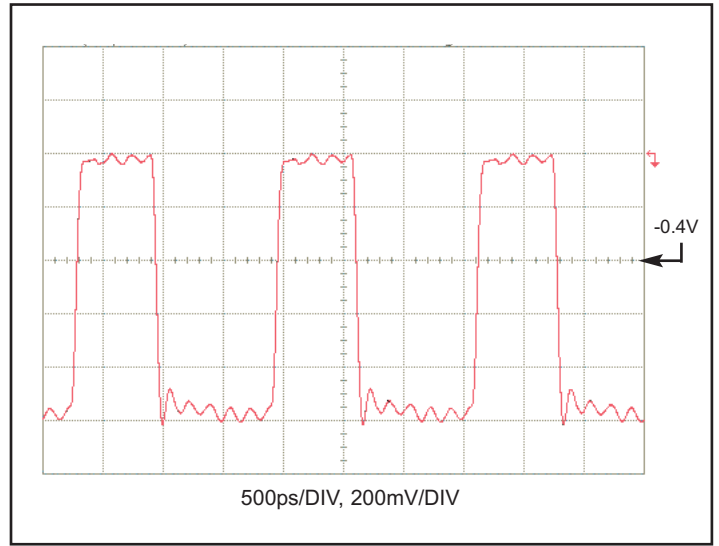
Waveform, Static Divide-by-10 Configuration Input Freq = 6 GHz, FRS=0
