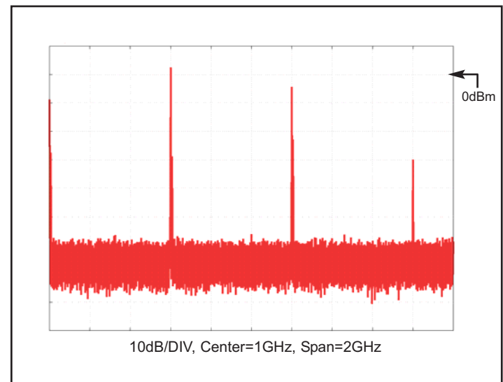
Spectrum, Static Divide-by-10 Configuration Input Freq = 6 GHz, FRS=0
