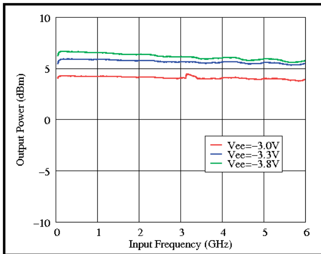
Output Power Divide-by-10, FRS=0
