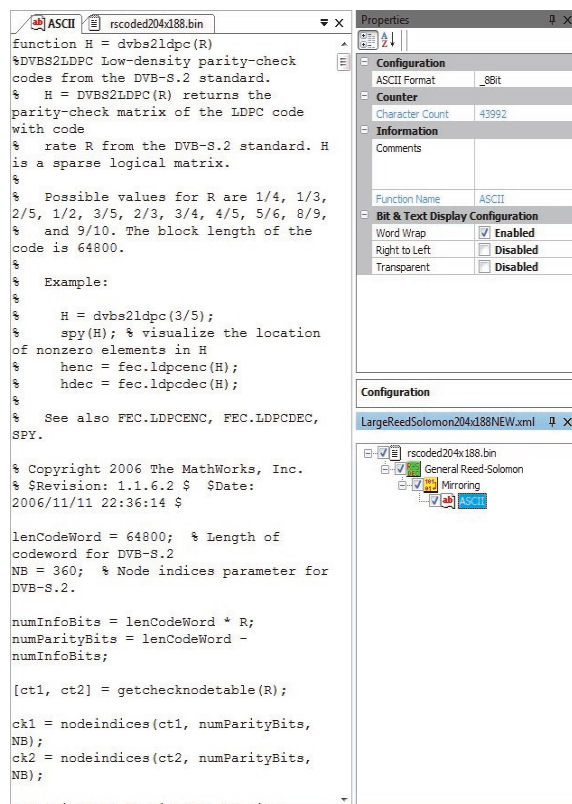
Reed-Solomon Example
