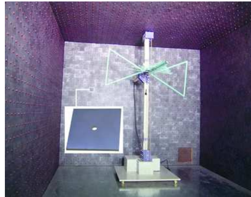
(7x3,8x3,6m EMC Anechoic Chamber)
