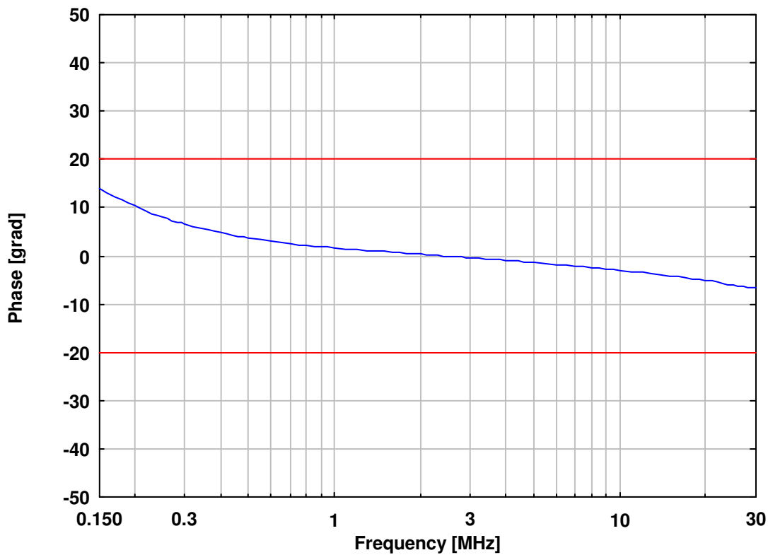
Fig.5b Common Mode Impedance (Phase) at EuT-Terminals (red lines: CISPR limits)
