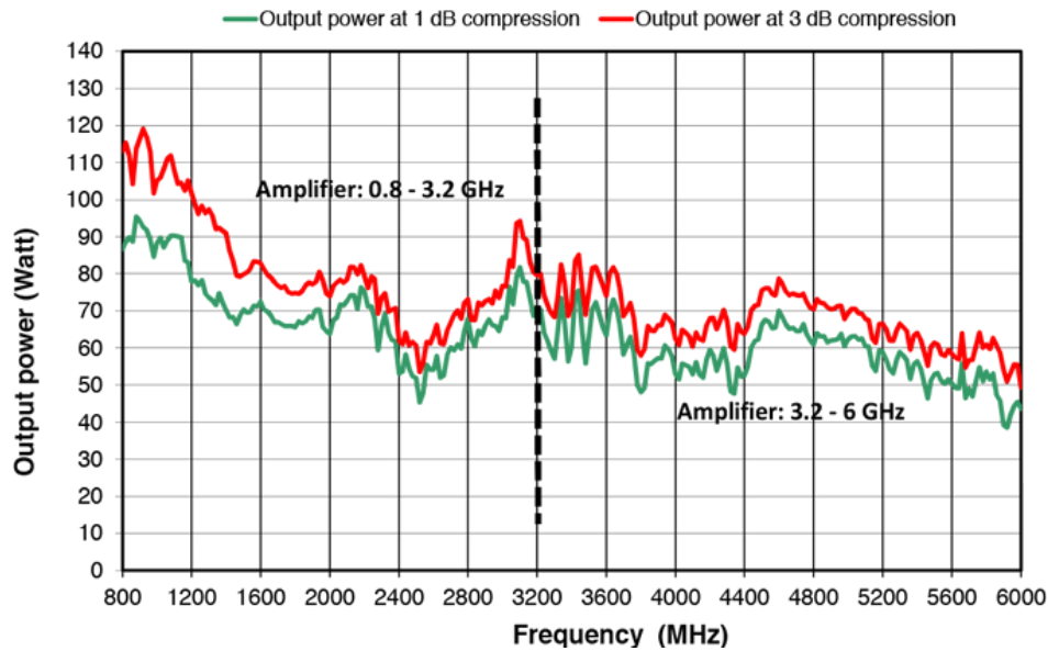
SX70/55 POWER AMPLIFIER 70W-55W / 800 MHz - 6000 MHz
