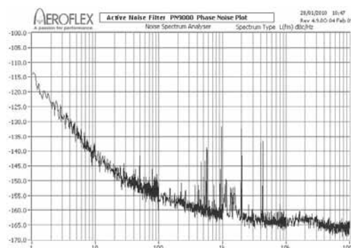
A6-ANF clean output oscillator performance Short term stability (AVAR) 5x10 -13 /s typically
