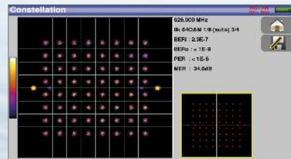
Constellation diagram in terrestrial, cable and satellite.
