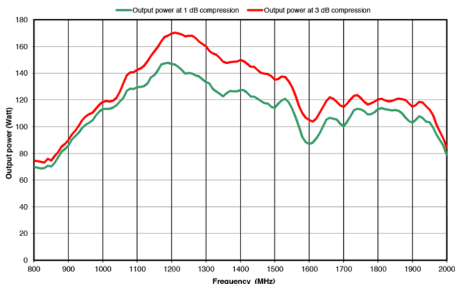
TU100 POWER AMPLIFIER 100W / 800 MHz - 2000 MHz
