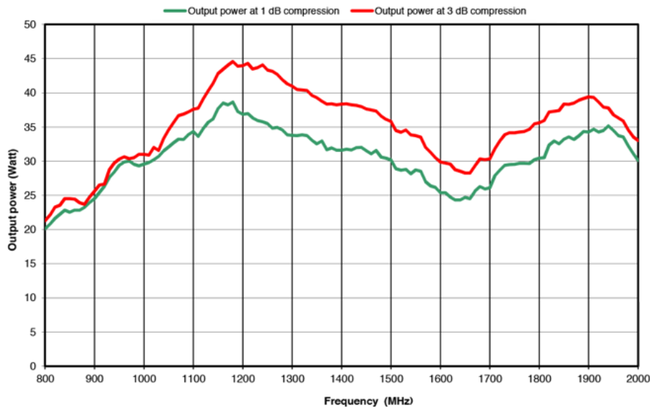
TU30 POWER AMPLIFIER 30W / 800 MHz - 2000 MHz
